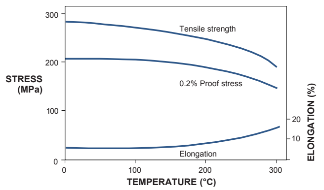
FIG. 1 Effect of temperature on tensile properties
