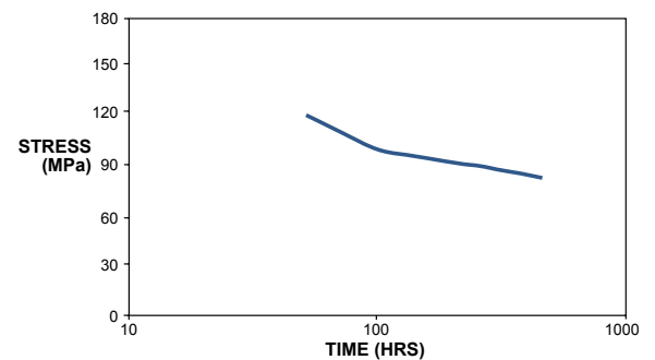
FIG. 2 Stress/time relationship at 200°C (0.1% creep strain)
