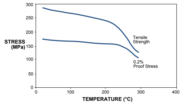
FIG. 1 Effect of temperature on tensile properties
